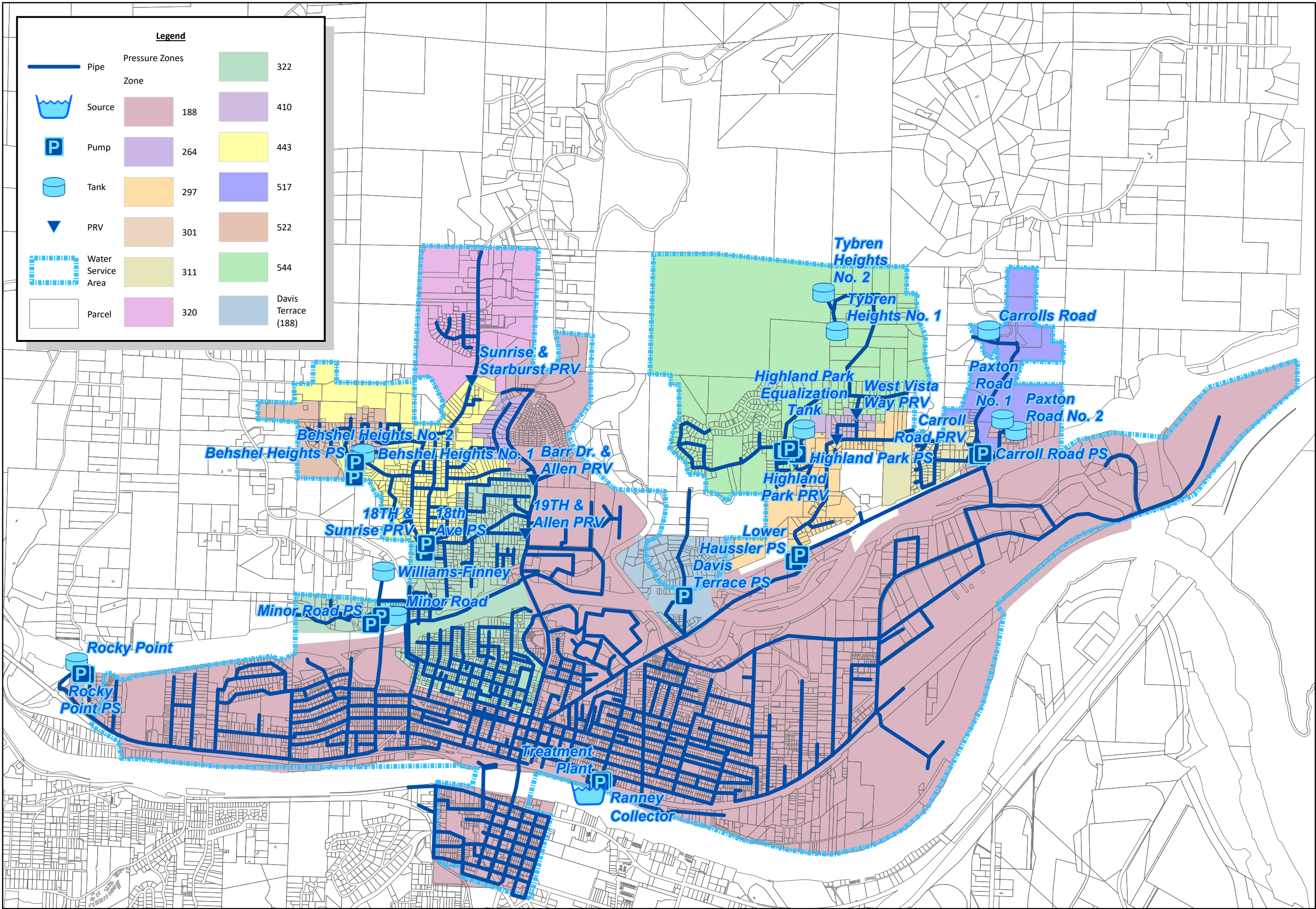
Figure 2.3 Existing Pressure Zones City of Kelso Water System Plan
