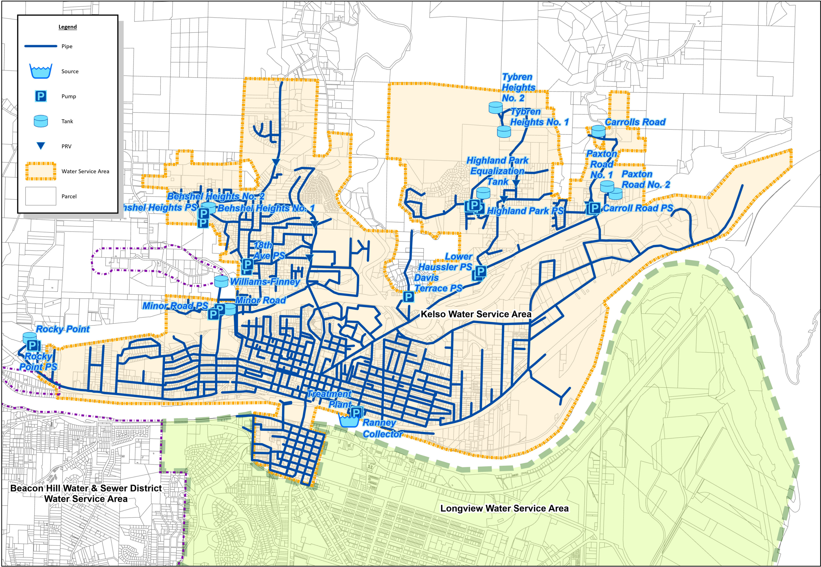
Figure 2.7 Adjacent Water Systems City of Kelso Water System Plan
