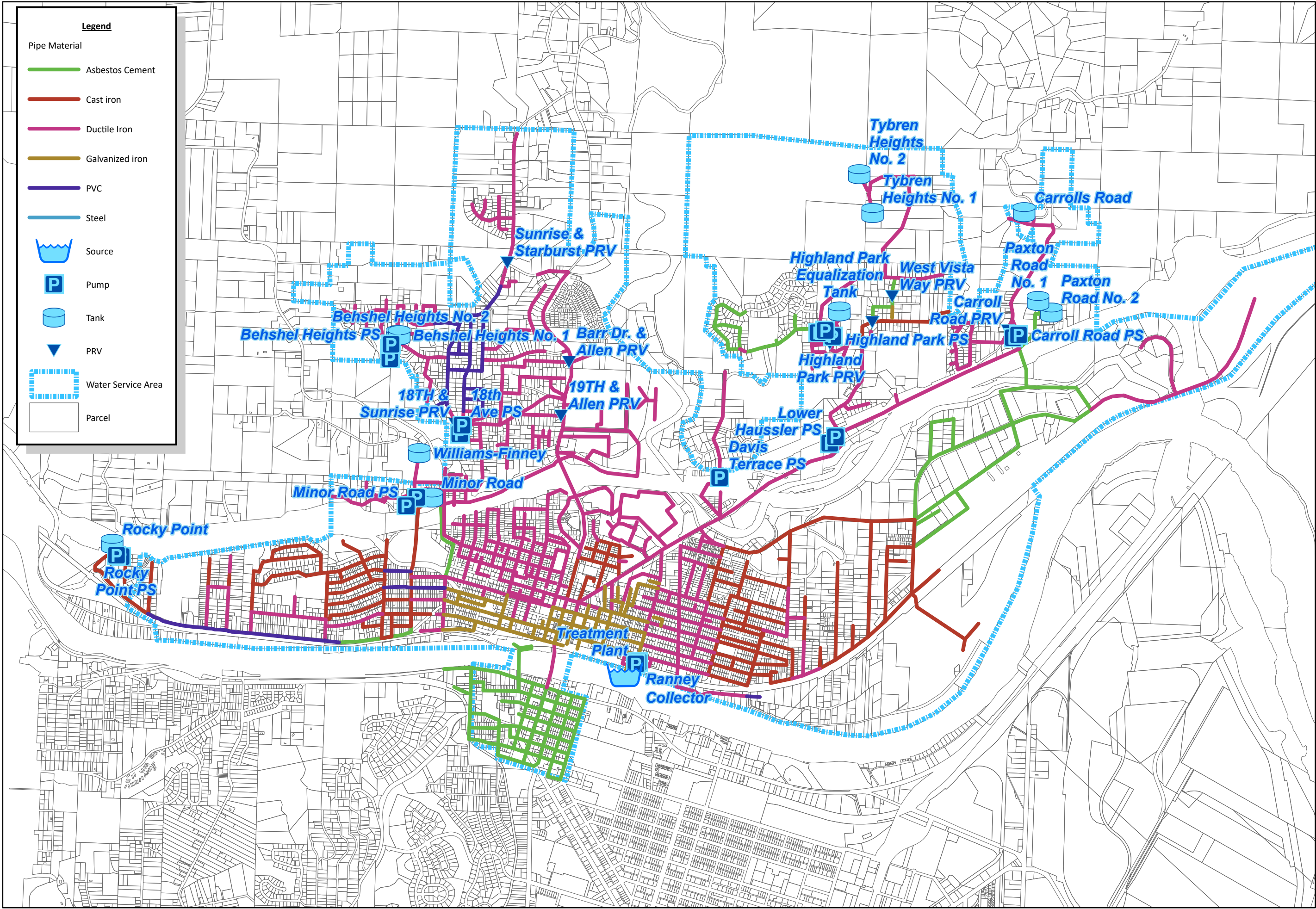
Figure 2.5 Existing Pipe Material City of Kelso Water System Plan
