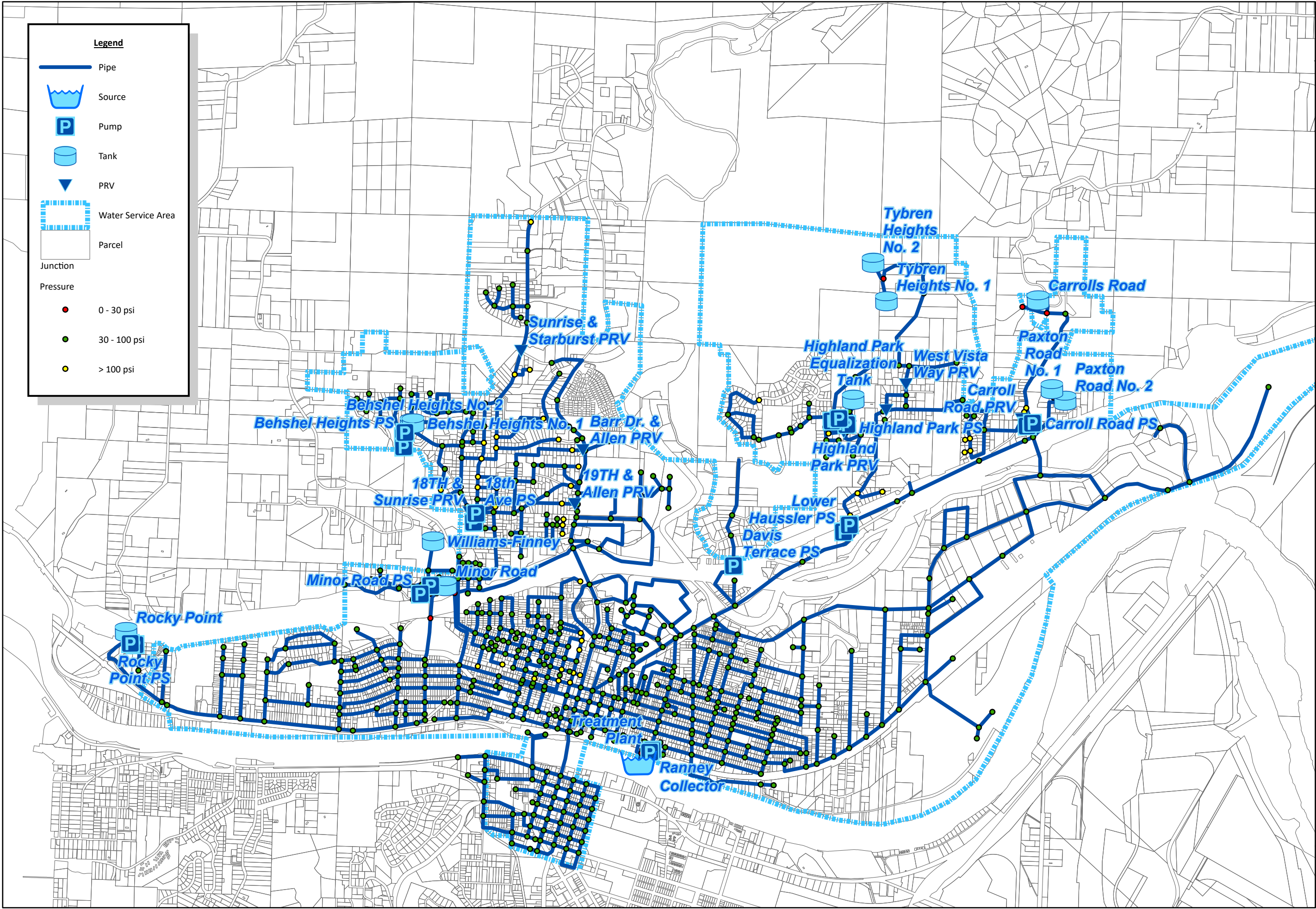
Figure B Existing Water System PHD City of Kelso Water System Plan
