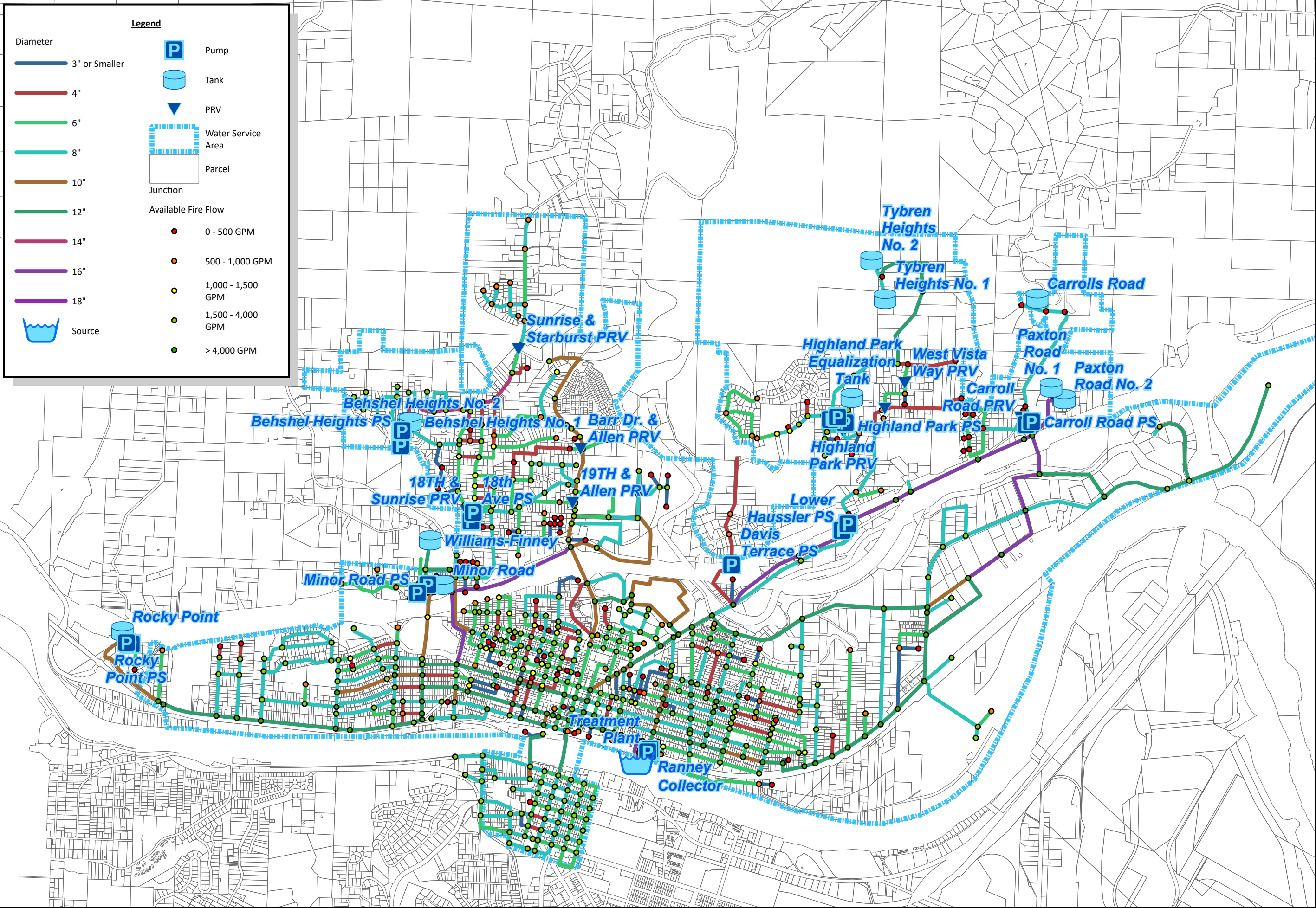
Figure E 2040 MDD Available Fire Flow City of Kelso Water System Plan
