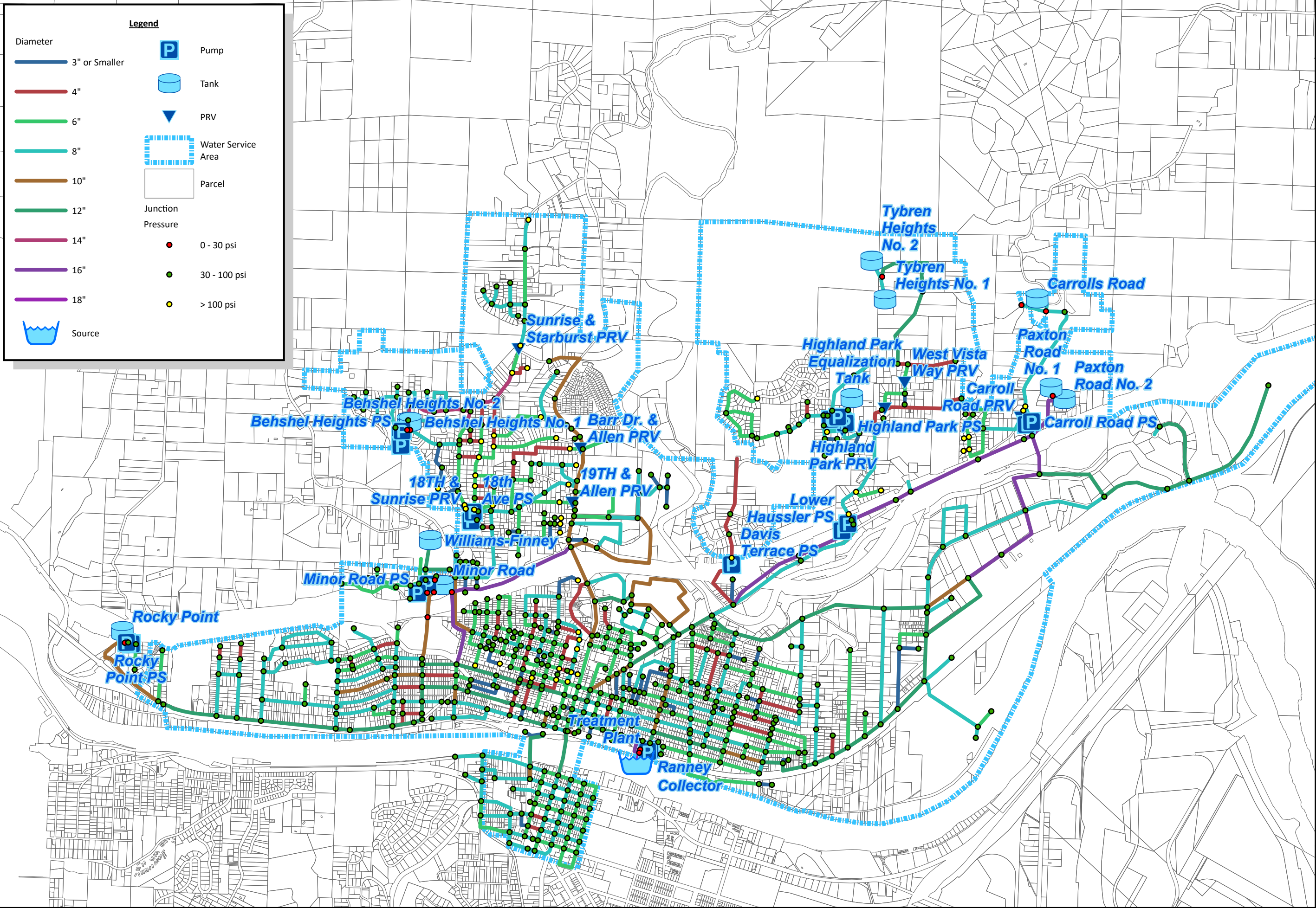
Figure D 2030 PHD Pressure City of Kelso Water System Plan
