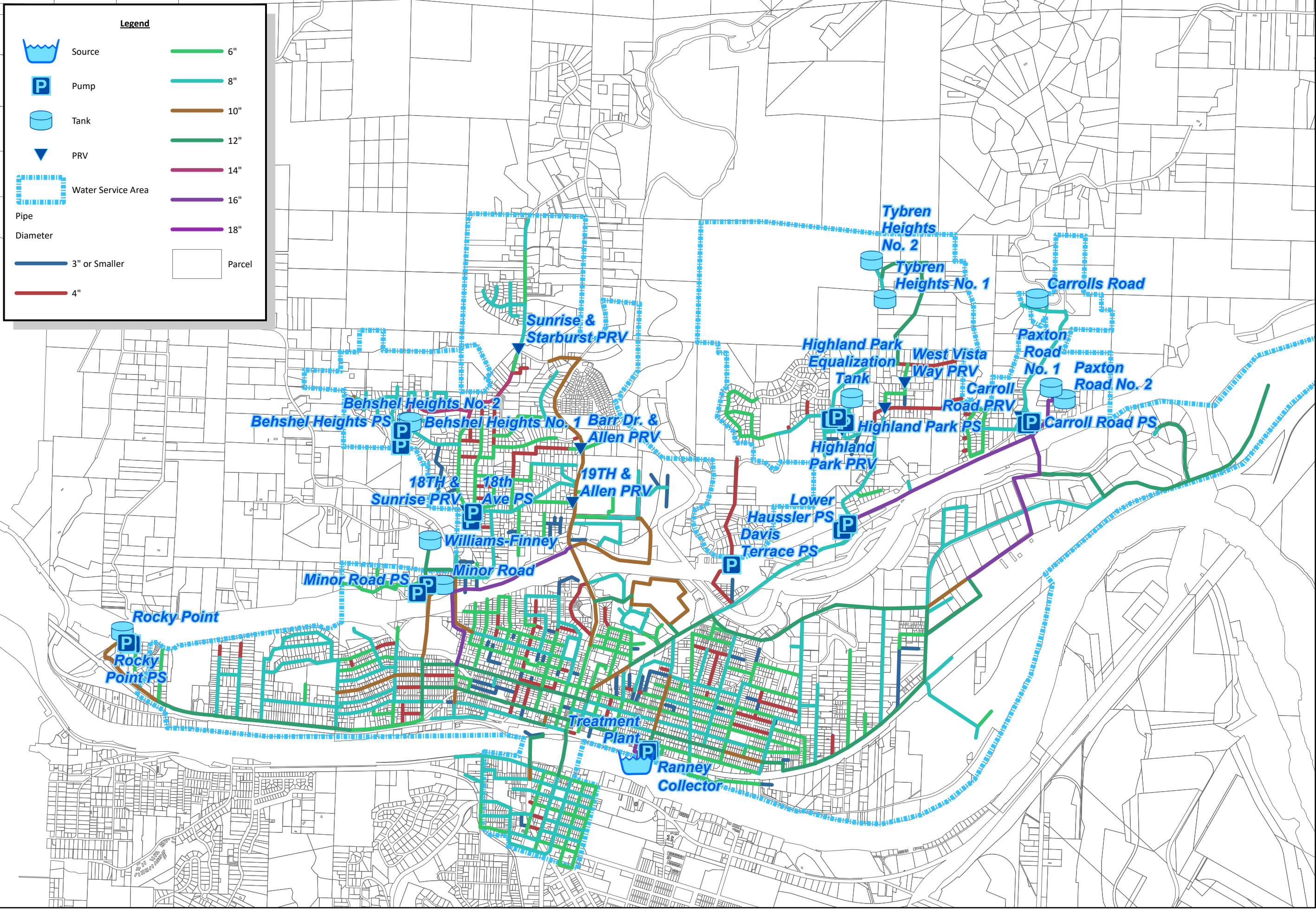
Figure 2.4 Existing Pipe Size City of Kelso Water System Plan
